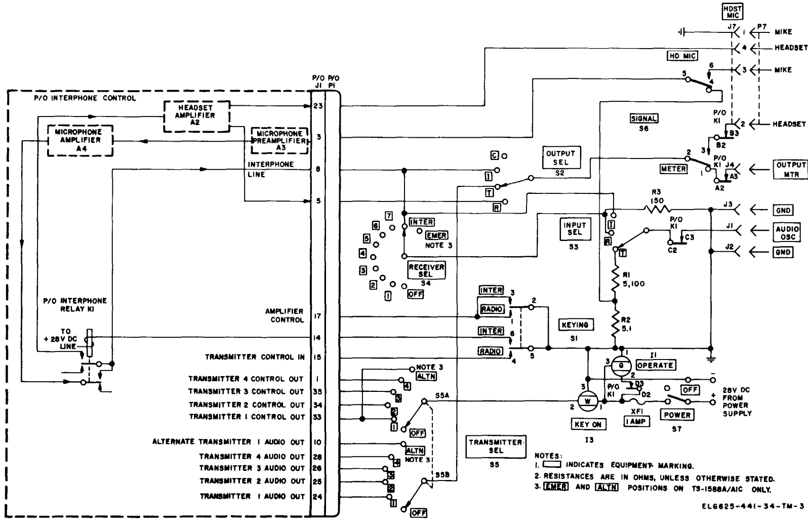
Figure 2-3. Interphone test set, transmission test circuits, simplified schematic diagram.
