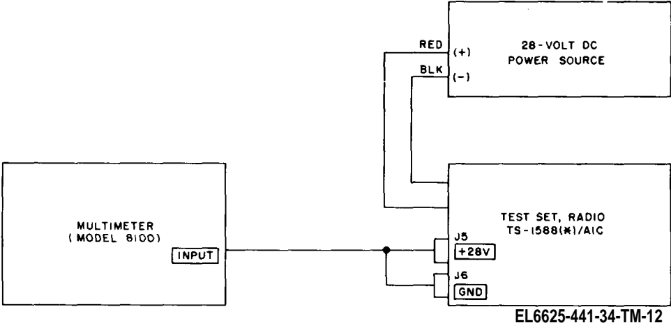
Figure 4-2. Test Set, Radio TS-1588(*)/AIC electrical test connection diagram.
